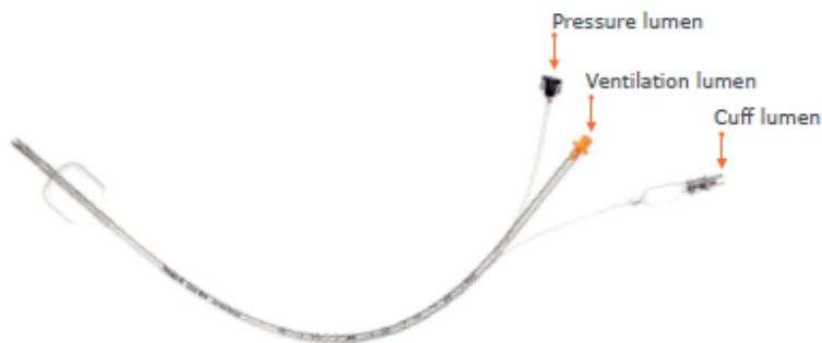
Tritube OD of only 4.4 mm (< 3 mm ID)
